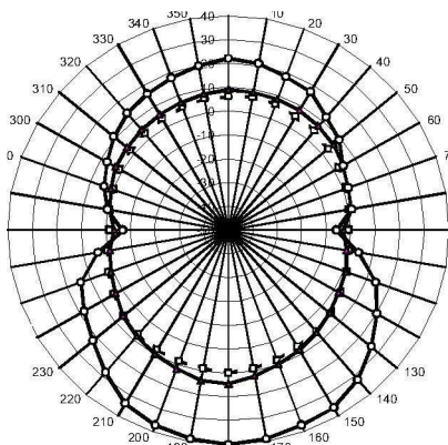
Figure 1 - Distribution of deformations of unirradiated and irradiated bodies on perimeter at pressure P = 14,5 MPa
