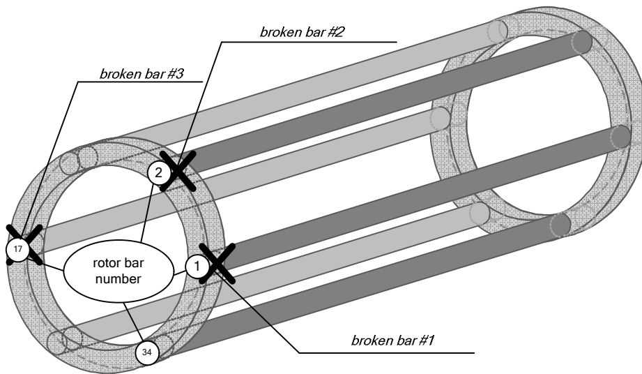
Figure 3 – Scheme of rotor apertures location: 1, 2, 3, 4 are broken bar numbers.
